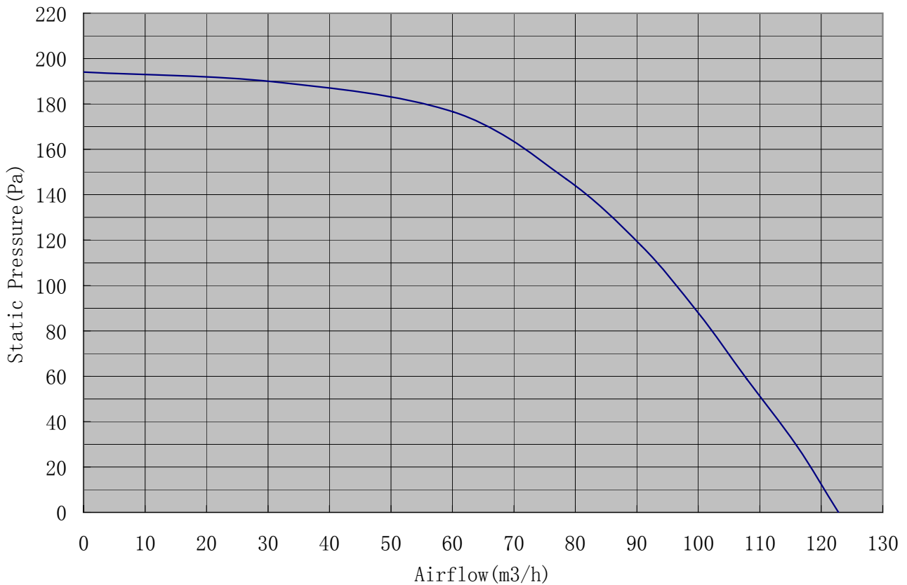
Airflow-Static Pressure Curve
